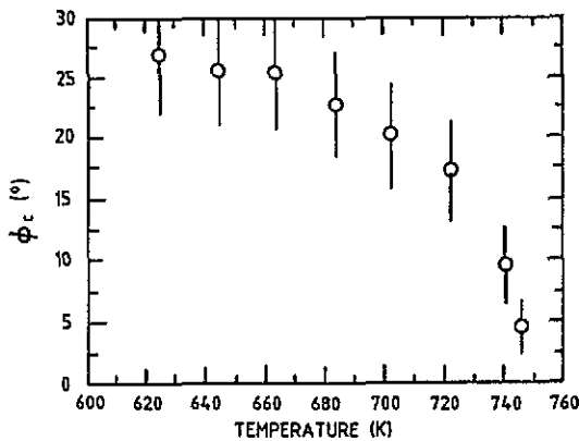
Figure 5. Temperature dependence of the \text{CO}_3 tilt angle, \phi_c .
