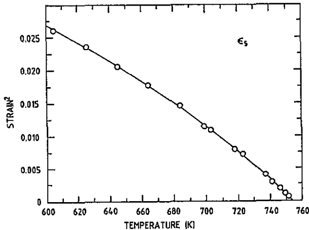
Figure 4. Temperature dependence of \epsilon_s^2 with the curve fitted using equation (23).
