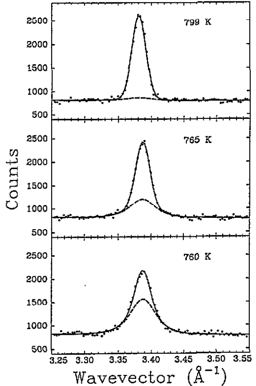
Figure 10. The temperature evolution of the line profile of the (202) peak above T_c . The broken line shows the exponential component, and the full line shows the complete analysed profile with the Bragg component included.
