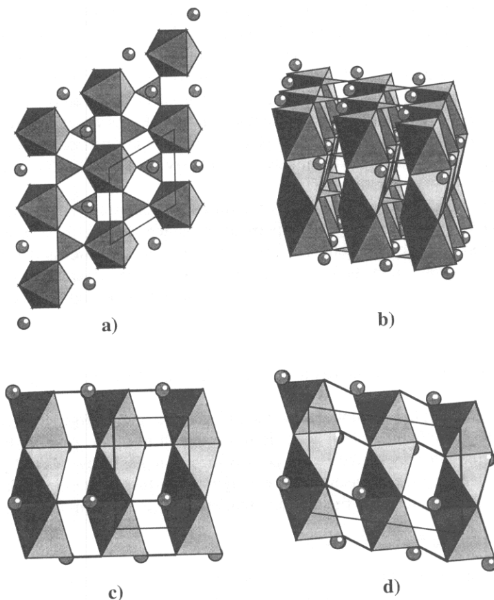
Figure 1. (a) Plan of the structure of the hexagonal \alpha -phase of sodium carbonate viewed down [001], showing the \text{Na(I)O}_6 octahedra and the carbonate groups (triangles). The position of the \text{Na(II)} atom is directly above the carbon atom, and is indicated by the shaded sphere. (b) Perspective view of the structure of the hexagonal \alpha -phase of sodium carbonate, showing the carbonate groups (triangles) acting as hinges connecting the columns of face sharing \text{Na(I)O}_6 octahedra. (c) Plan of the structure of the hexagonal \alpha -phase of sodium carbonate viewed down [010], for comparison with (d). The thick lines indicate the planes of the carbonate groups. (d) Plan of the structure of the monoclinic \beta -phase of sodium carbonate viewed down [010]. In this projection the shear strain and the coupled hinged rotations of the carbonate groups are clear, particularly when compared with the view of the hexagonal phase from the same direction, (c).
