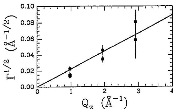
Figure 14. The dependence of \Gamma_{(h k \ell)}^{1/2} on Q_z determined at 756 K. The straight line is the result of a least-squares fit through the origin.
